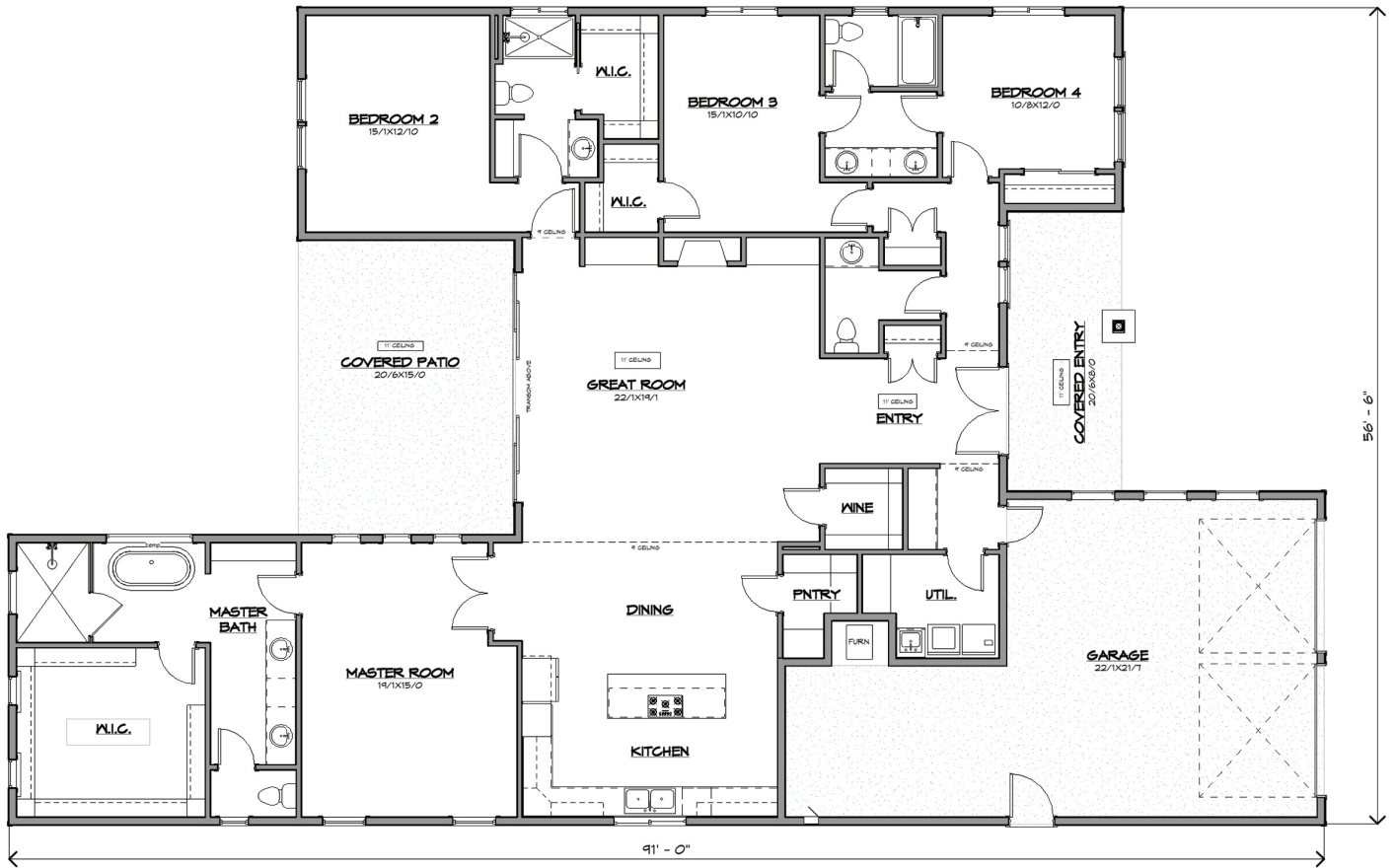
Main Floor Plan - 2792 SF
