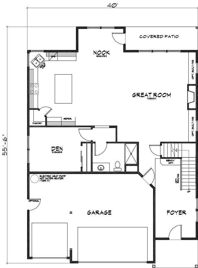
MAIN FLOOR 3080
