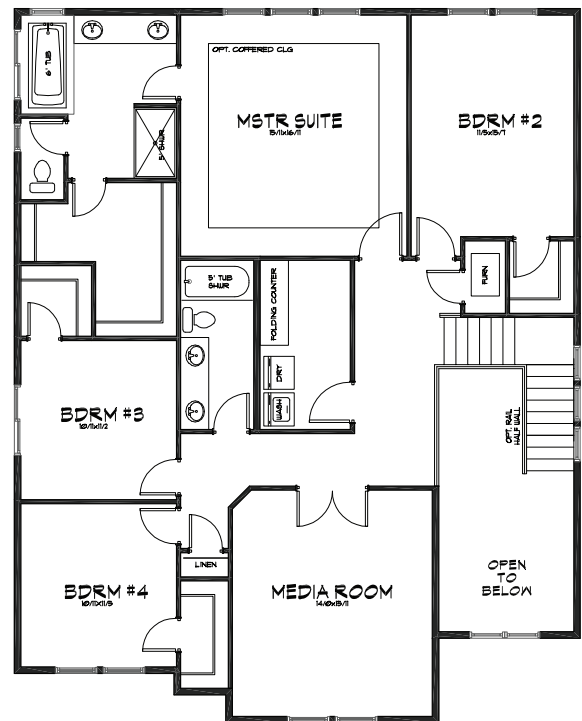
UPPER FLOOR 3080
