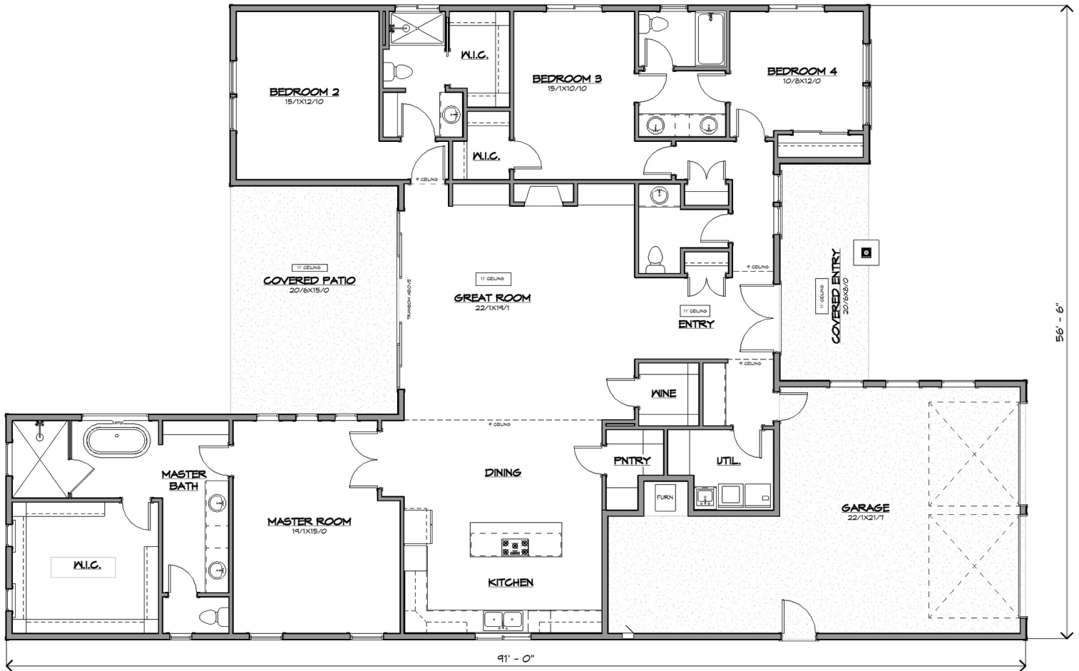
Main Floor Plan - 2792 SF
